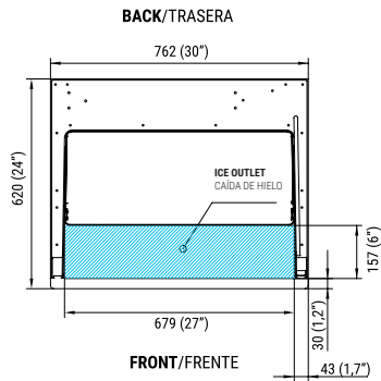
CENTRAL CROSS SECTION VIEW OF THE BASE
